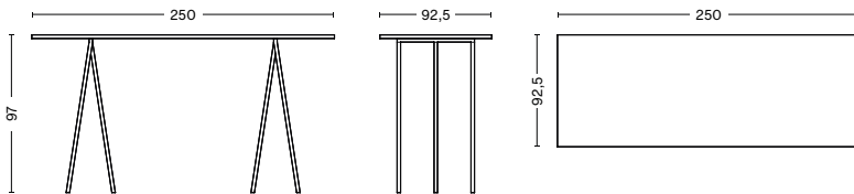
LOOP STAND HIGH L250 LENGTH 250 CM WIDTH 92,5 CM HEIGHT 97 CM
